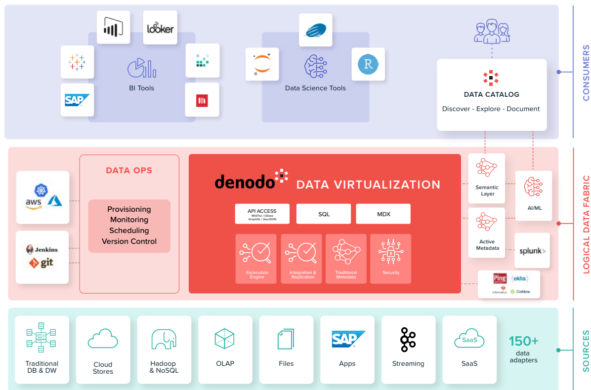
Figure 2: Functional diagram of a Logical Data Fabric
