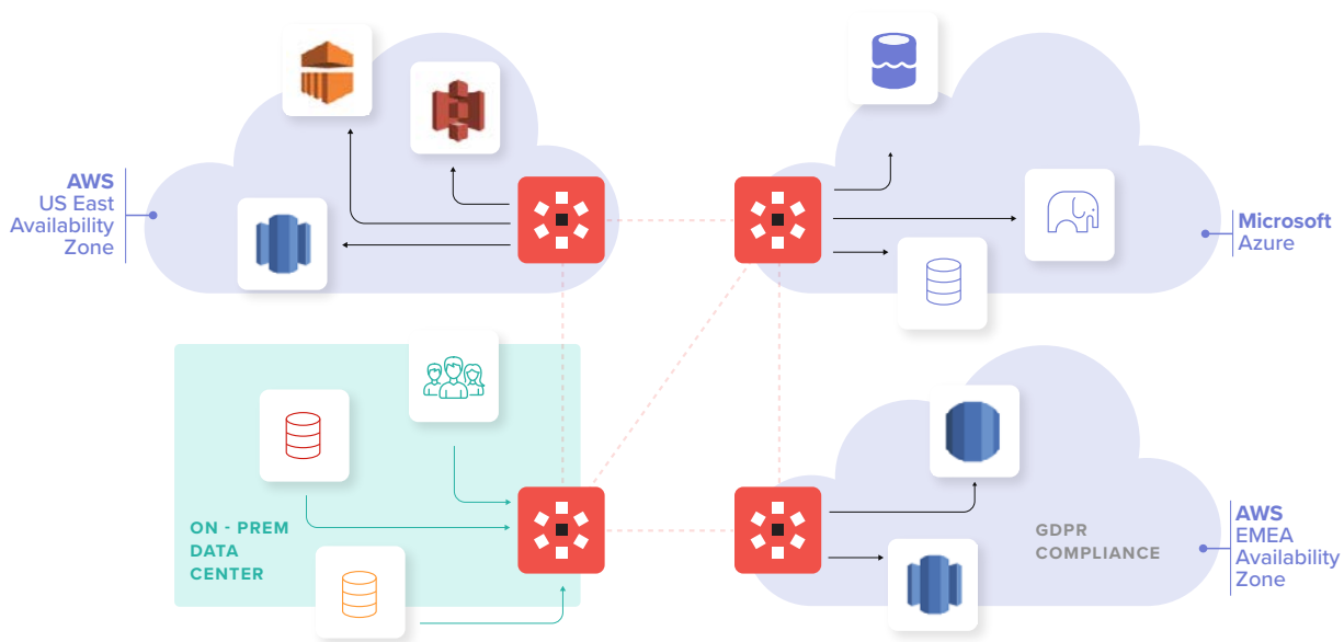
Figure 3: Multi-Cloud Provisioning
